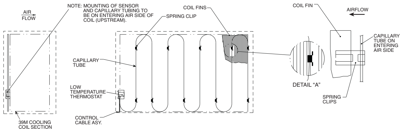
Fig. 23 — Cooling Coil Section, Capillary Tube Routing
