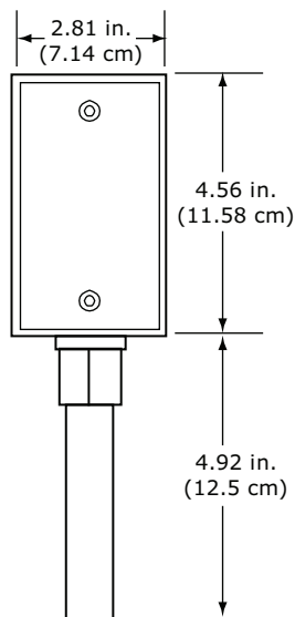
Fig. 19 — Outdoor-Air Temperature (OAT) Sensor
