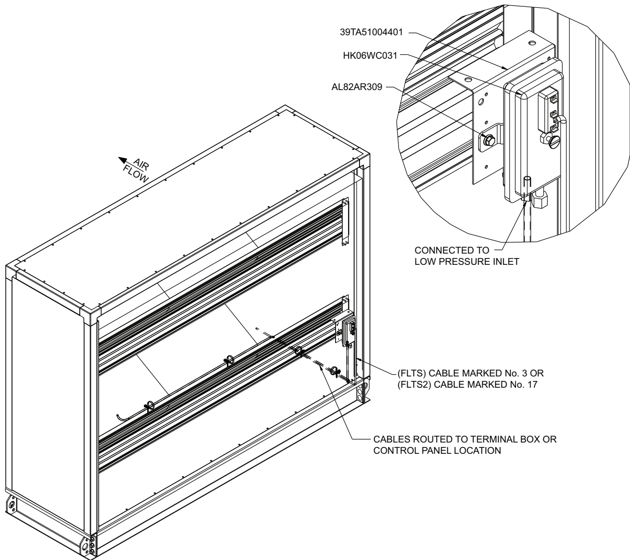
Fig. 24 — Filter Status Switch Installation
