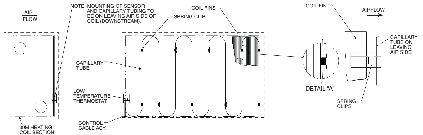
Fig. 22 — Heating Coil Section, Typical Capillary Tube Routing for LTT on Heating Only Applications
