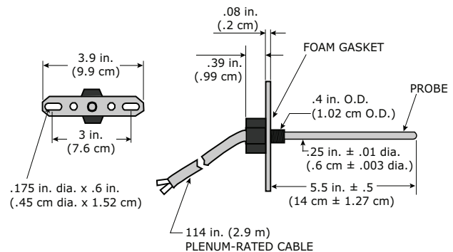
Fig. 14 — Supply-Air/Return-Air Temperature Sensor (33ZCSENSAT)
