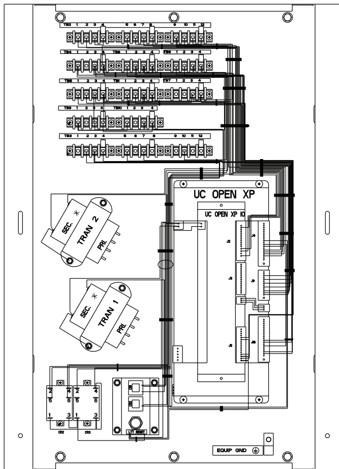
Fig. 4 — UC Open XP Control Box Components
