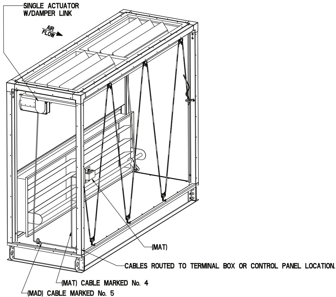
Fig. 20 — Typical MAT (Mixed-Air Temperature Sensor) Installation
