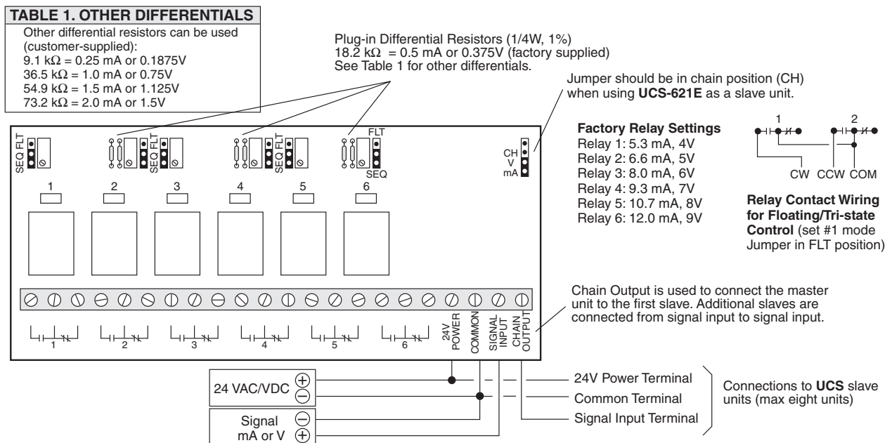
Fig. 27 — 6-Stage Electric Heat Sequencer
