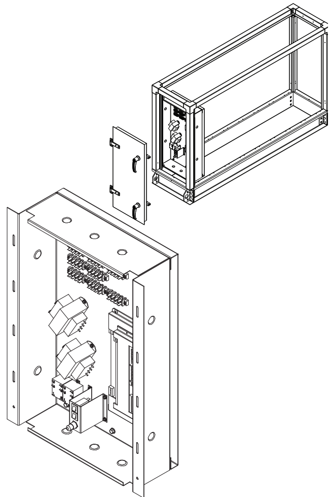
Fig. 1 — Typical Control Box Installation on 39M Supply Fan Section
