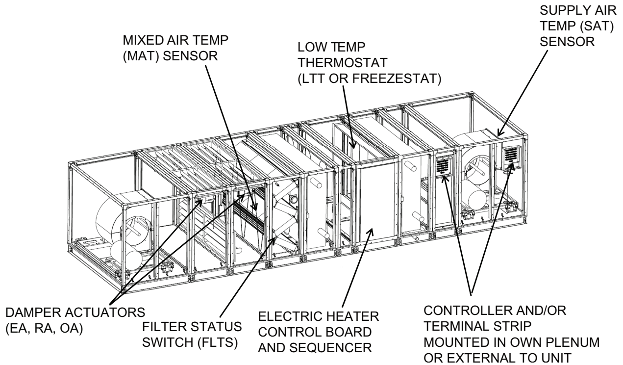
Fig. 2 — 39M Typical Sensor, Actuator, and Controller Installation Locations
