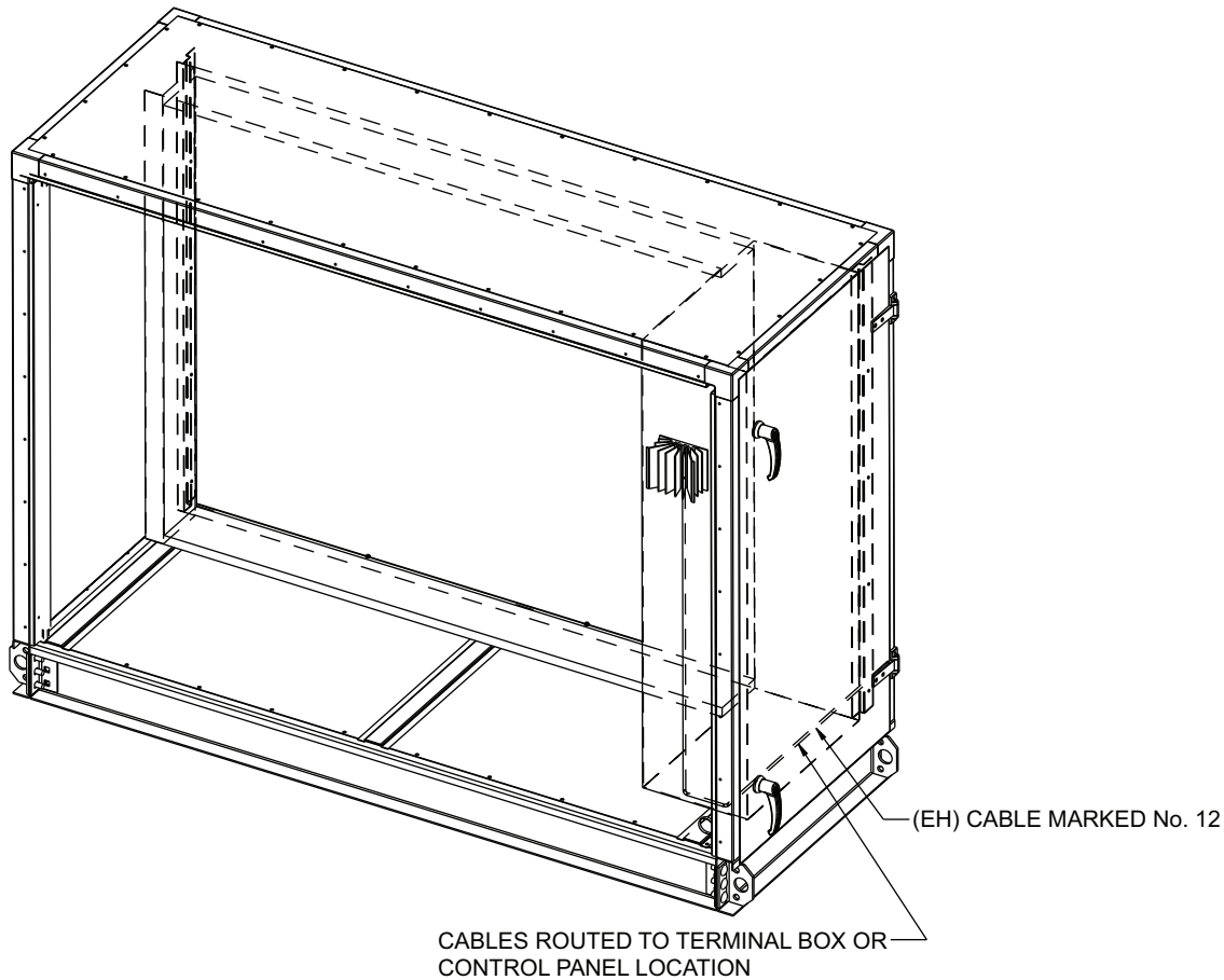
Fig. 28 — SCR Installation
