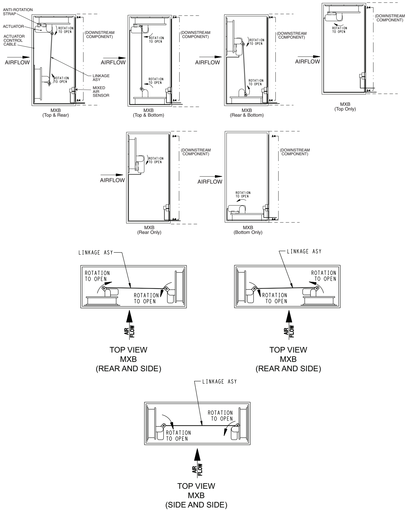
Fig. 26 — Actuator Field Mounting
