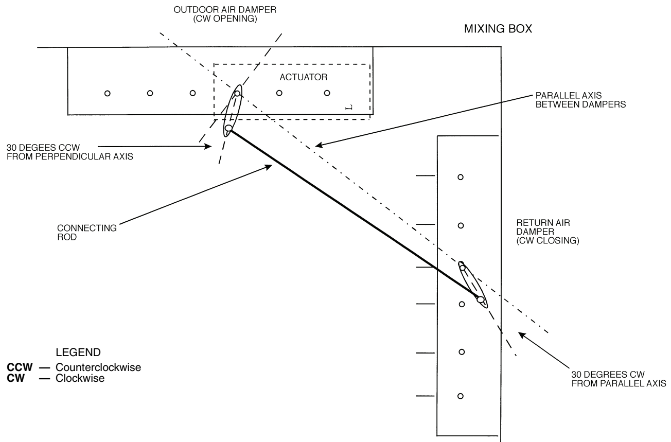
Fig. 25 — Typical Damper Secondary Linkage (Two Parallel Blade Dampers)
