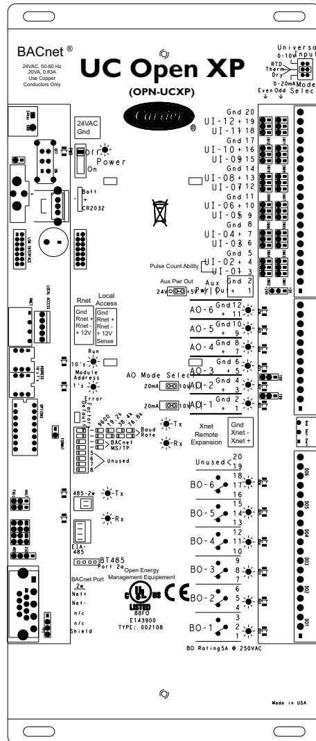
Fig. 7 — UC Open XP Input and Output Terminals
