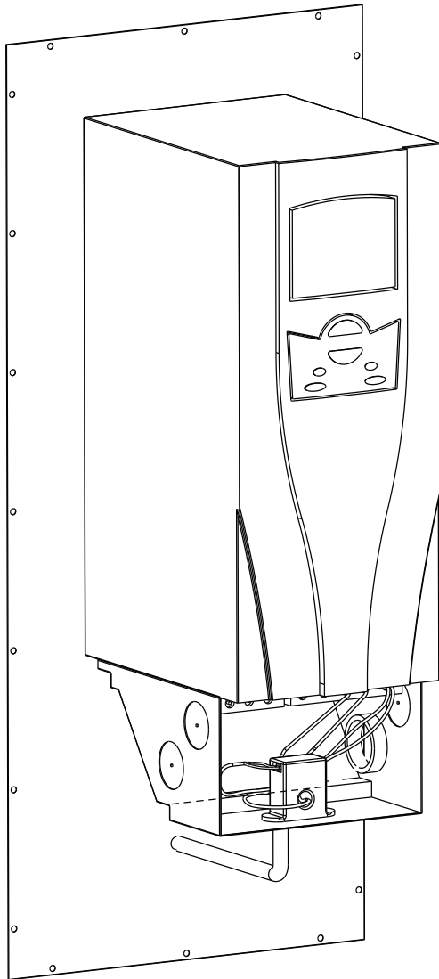
Fig. 16 — Fan Status Switch Installed in VFD
