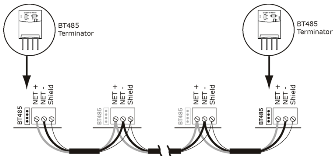
Fig.10 — UC Open XP Communication Wiring
