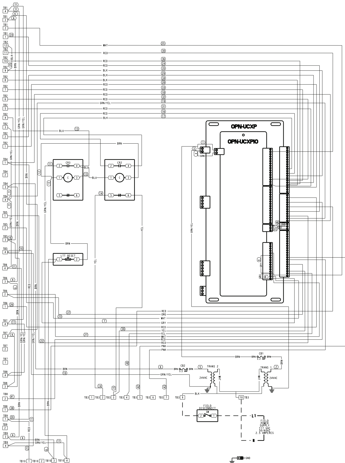
Fig. 6 — Controller Wiring Schematic
